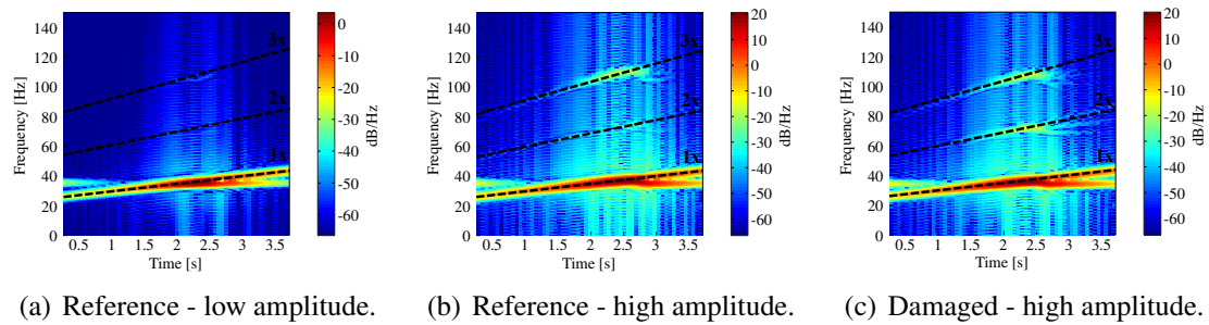
Figure 2: Time-frequency diagram of the system's output exemplifying the presence of nonlinear phenomena.
