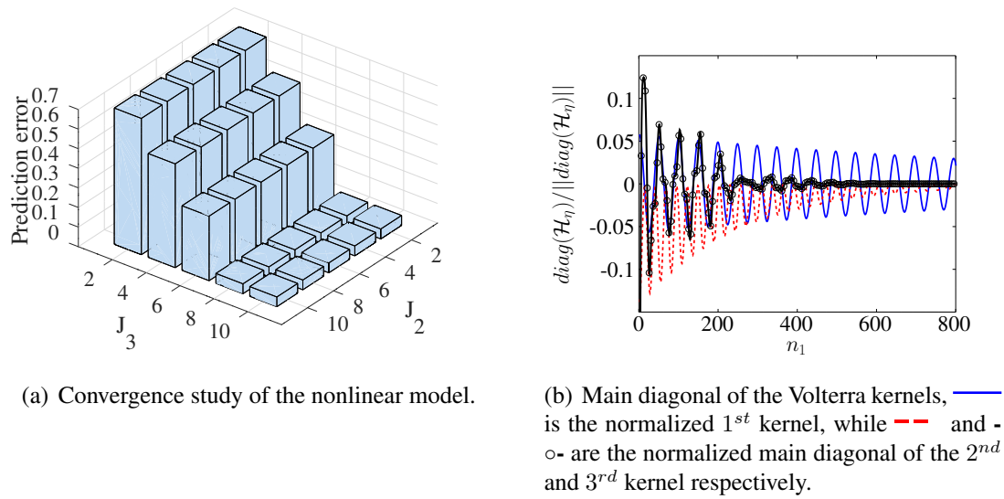
Figure 5: Volterra model representing the MAGNOLIA system.
