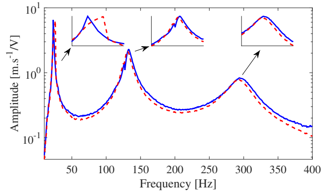
(b) Stepped sine response. — and - - - represents the response to an input of 0.01 V and 0.15 V respectively.
