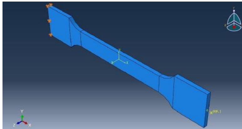
Figure 8 - Model with boundary conditions and loading
