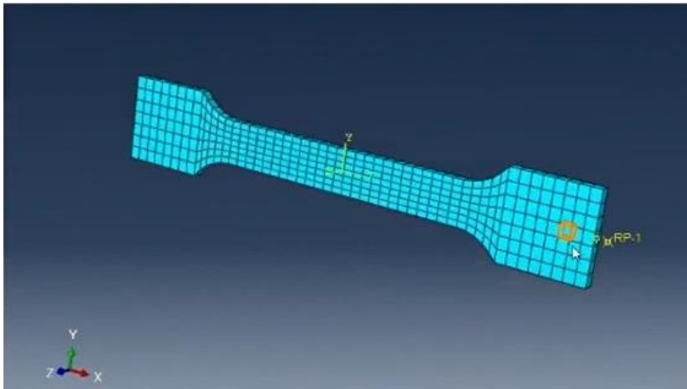
Figure 9 - Mesh applied to the model
